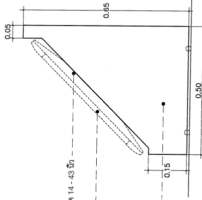
ELEVATION B SCALE 1 : 15
