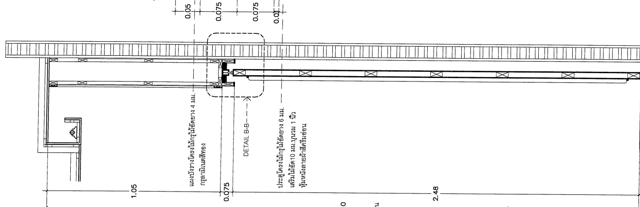
PLAN SCALE 1:25
