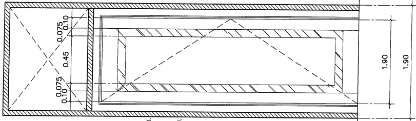
DETAIL D-D SCALE 1:25
